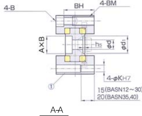
Provides extension of slide part by 5mm
